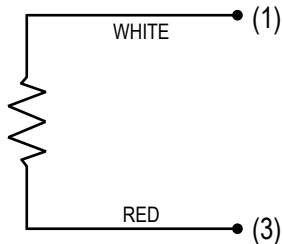
2-Wire
