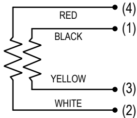
Dual 2-Wire
