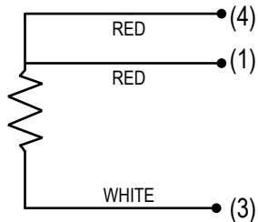
3-Wire
