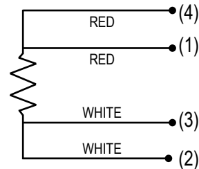
4-Wire
