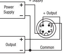
3 WIRE WIRING DIAGRAM EXAMPLE
