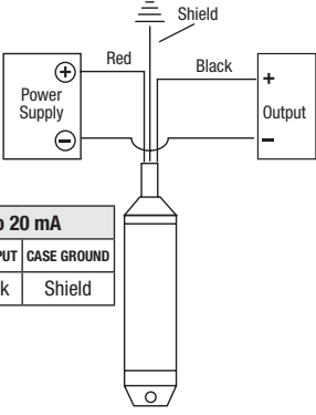
2 WIRE WIRING DIAGRAM EXAMPLE
